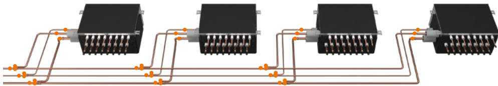
VRV IV+: 39 brazing points and 3 joint kits
